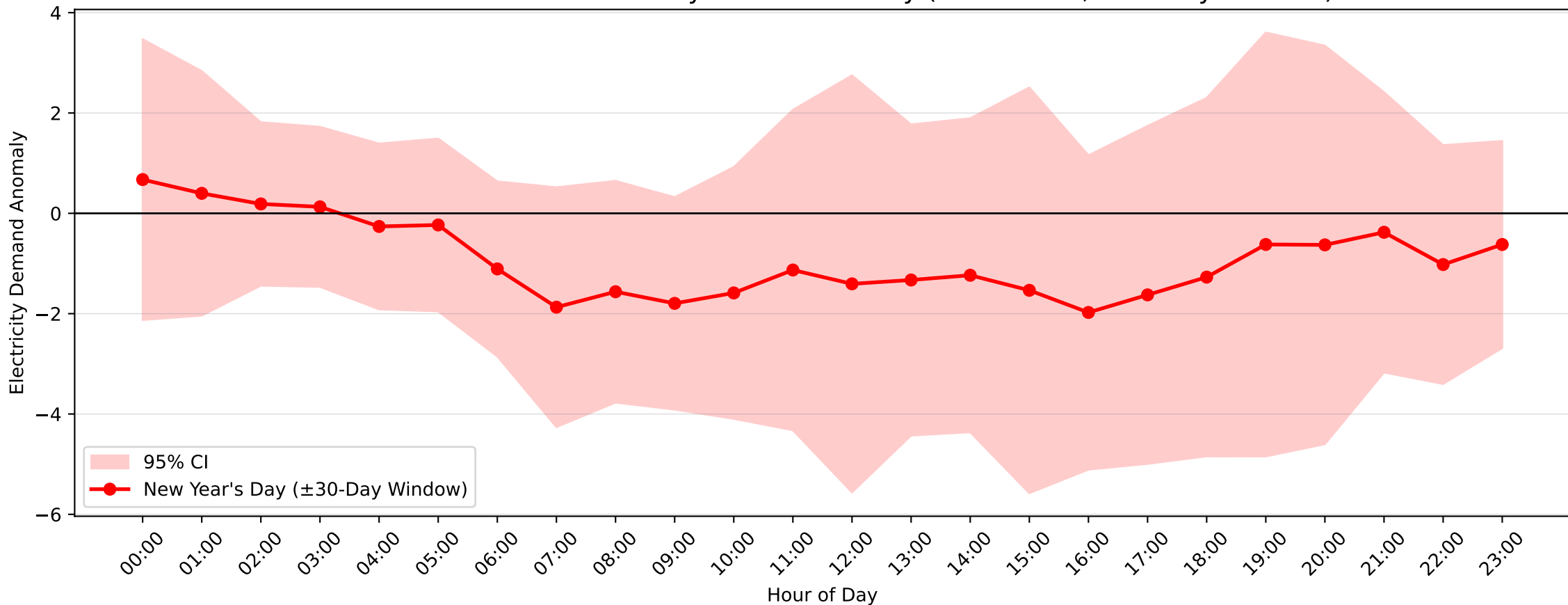
Adamstown Demand Anomaly: New Year's Day (2004-2017, \pm 30 -Day Window)
